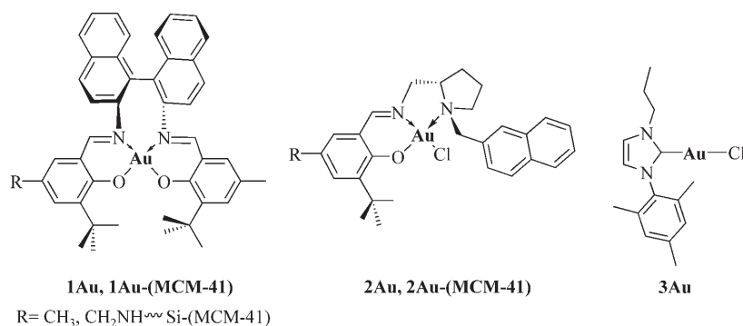
Figure 1. Gold compounds studied as hydrosilylation catalysts.
